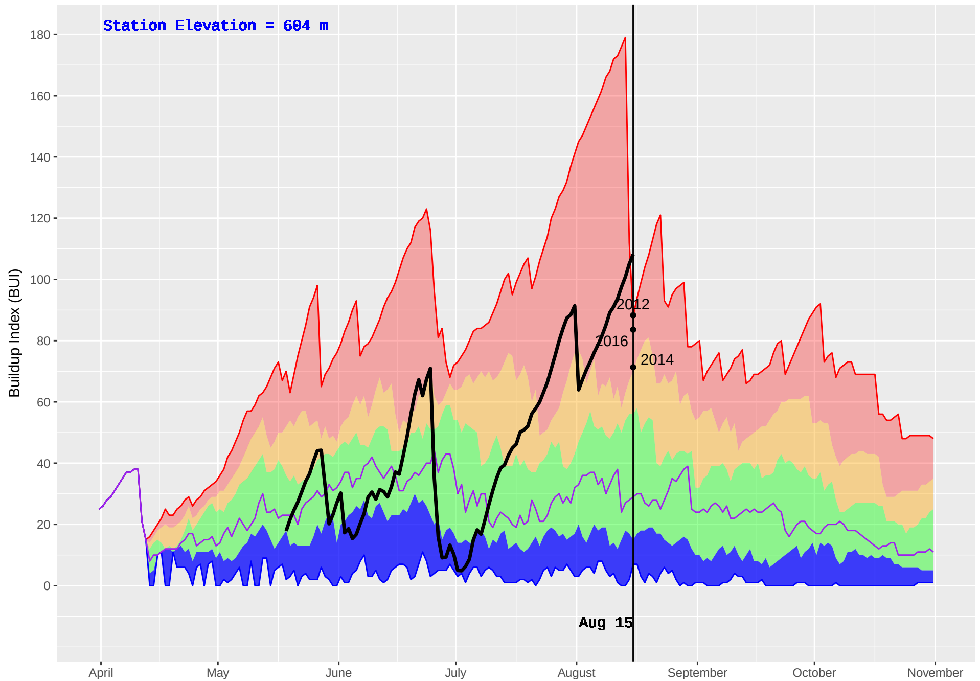
NELSON FORKS (119) : Historical (1986–2016) and Current (2018) Daily Buildup Index (BUI)
