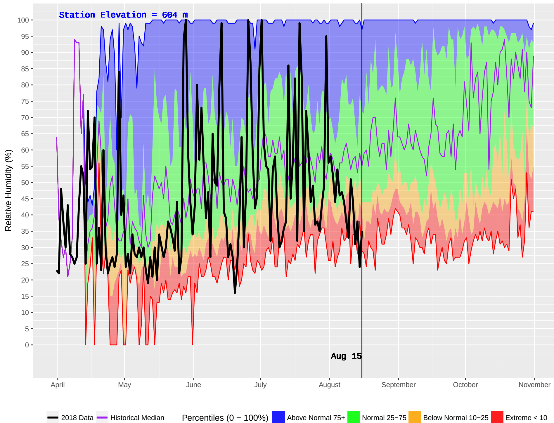
NELSON FORKS (119) : Historical (1986–2016) and Current (2018) Daily Relative Humidity
