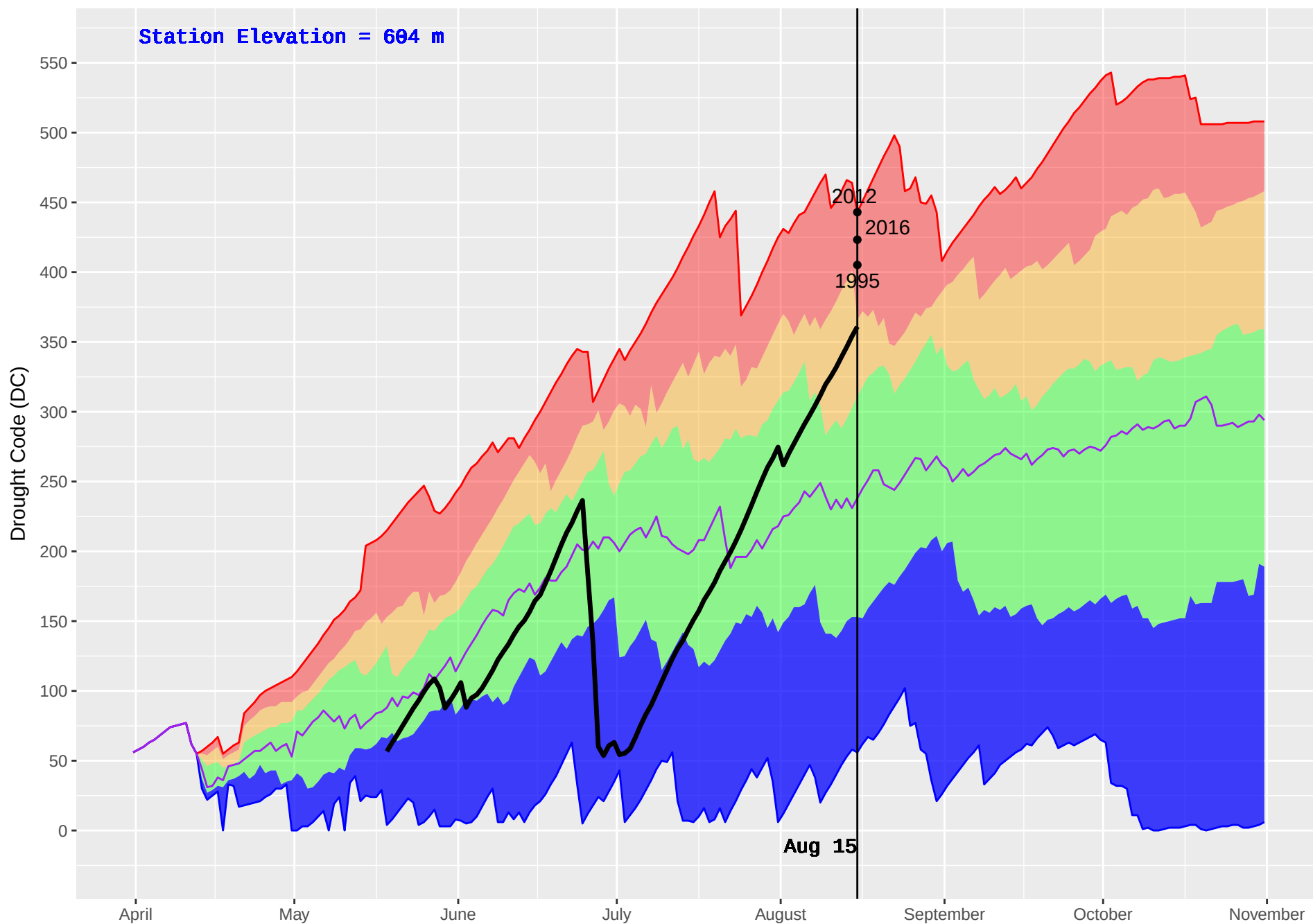
NELSON FORKS (119) : Historical (1986–2016) and Current (2018) Daily Drought Code (DC)
