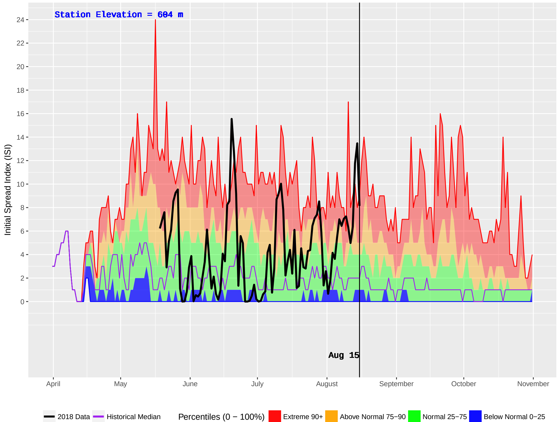
NELSON FORKS (119) : Historical (1986–2016) and Current (2018) Daily Initial Spread Index (ISI)
