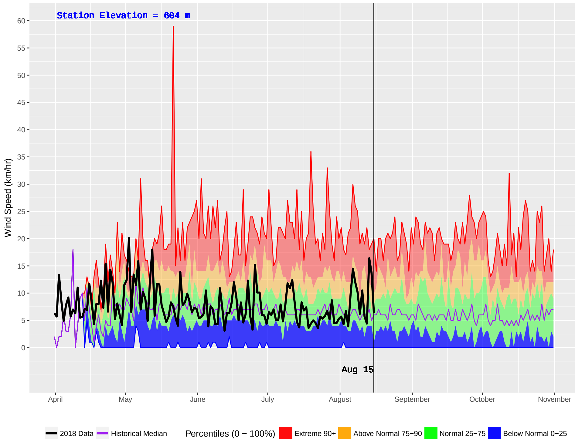
NELSON FORKS (119) : Historical (1986–2016) and Current (2018) Daily Wind Speed
