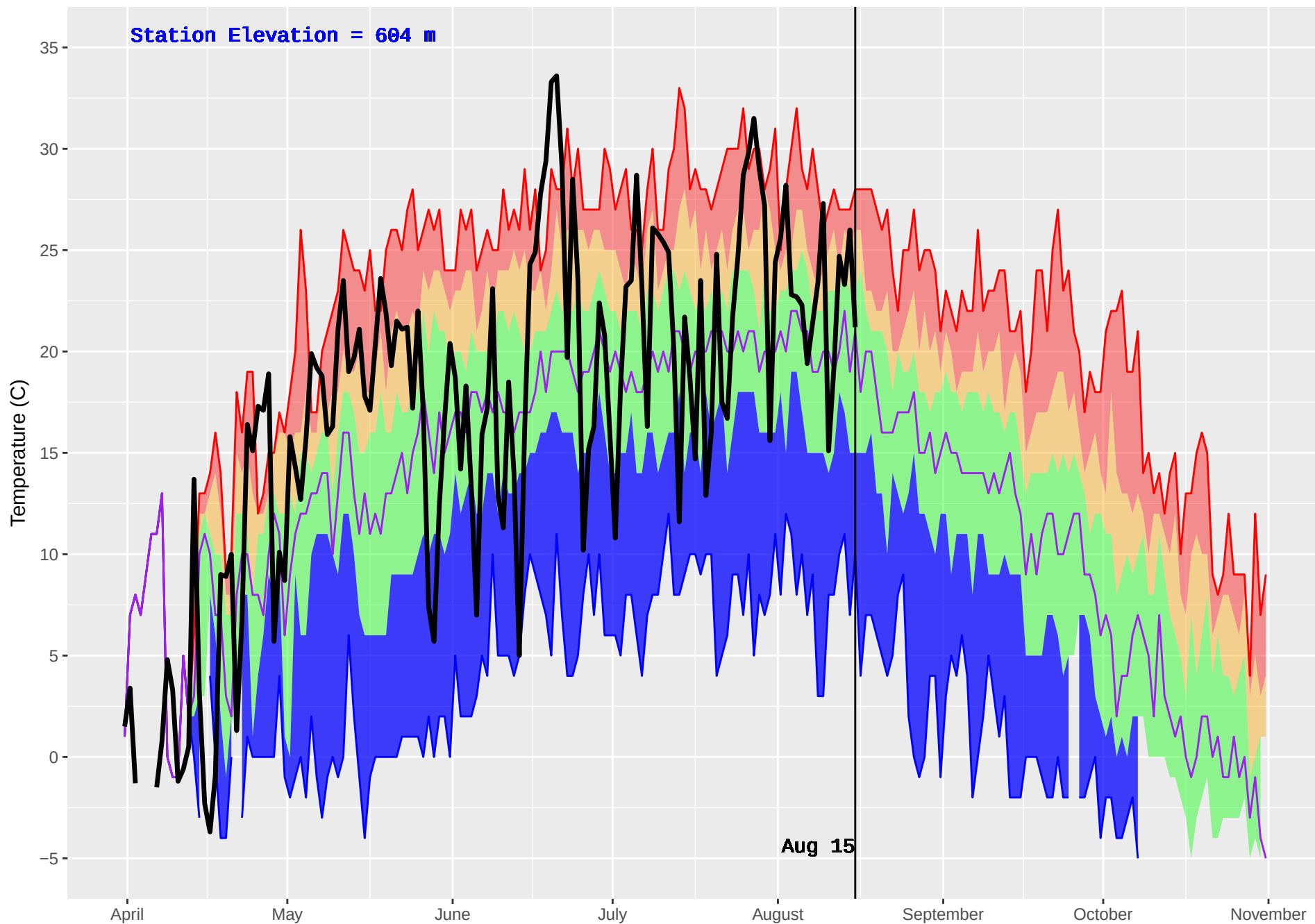
NELSON FORKS (119) : Historical (1986–2016) and Current (2018) Daily Temperature
